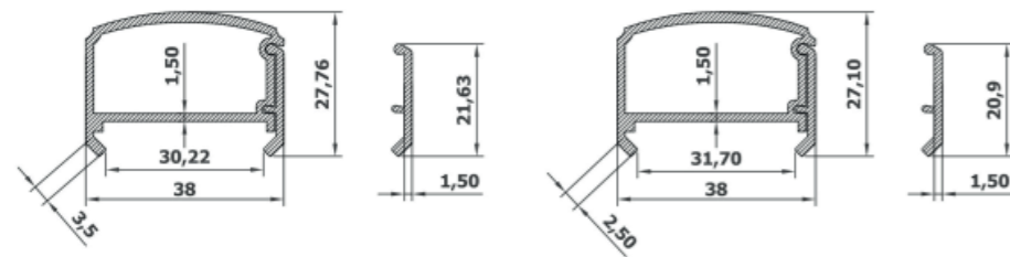
Continuous horizontal profile / Perfil horizontal continuo
